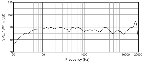
Measured on-axis with distance referenced to 1 meter at 1 watt, half-space (128W)
